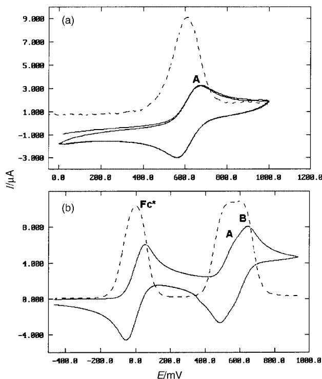
Fig. 3 Cyclic and square wave voltammograms of (a) compound 6 and (b) 4 in CH 2 Cl 2 , Pt, 0.1 M n Bu 4 NPF 6 , 100 mV s -1 .
